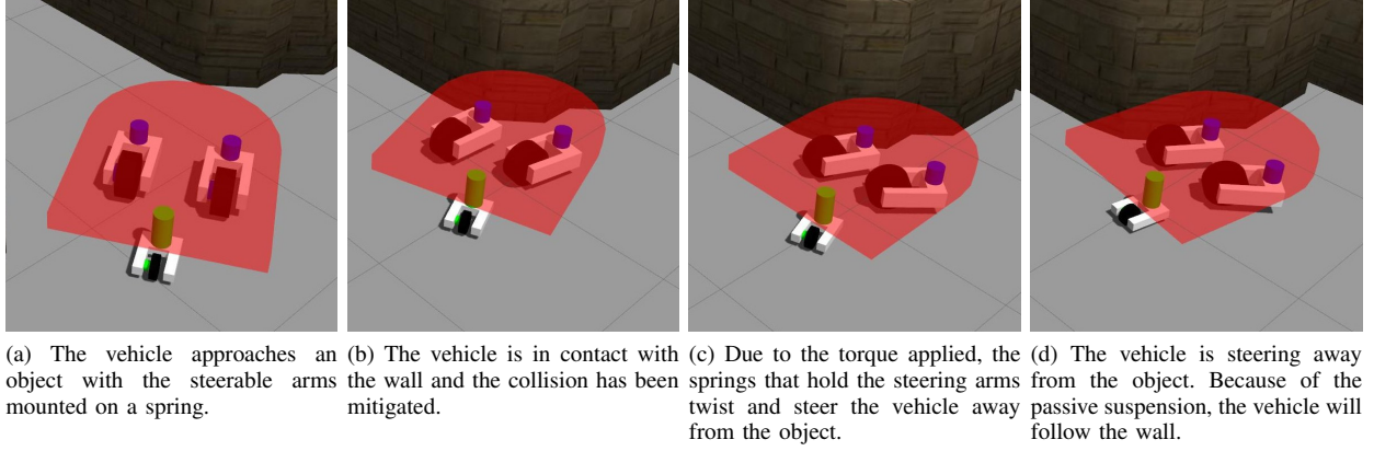
Fig. 8: Collision mitigation and recovery. An IWOS vehicle is capable of mitigating the collision and leading the vehicle away from the contact point.
