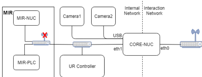
Fig. 3. Network architecture
