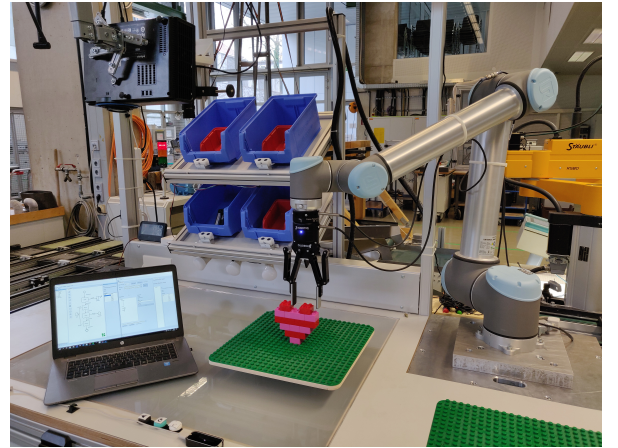
Fig. 4. Demonstration setup.
