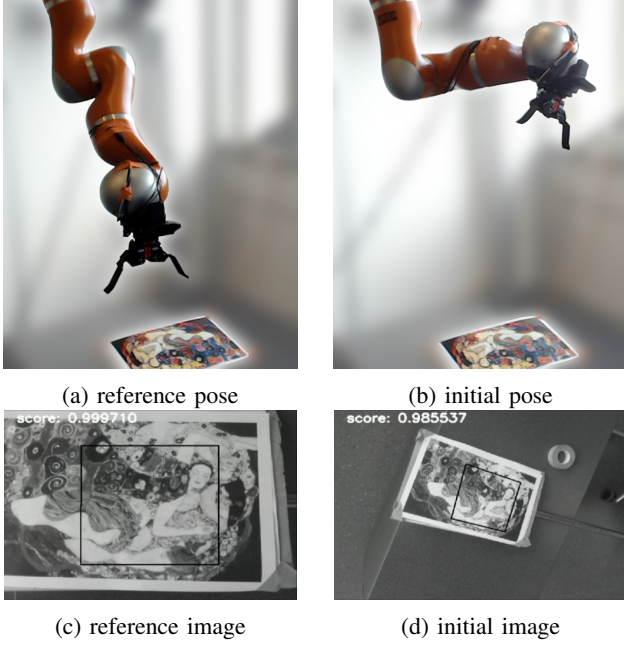
Fig. 3: Positioning Experiment
