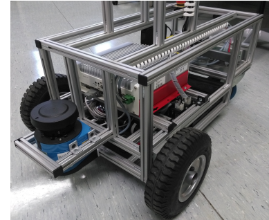
Fig. 1. Mobile Robot "Volksbot"
