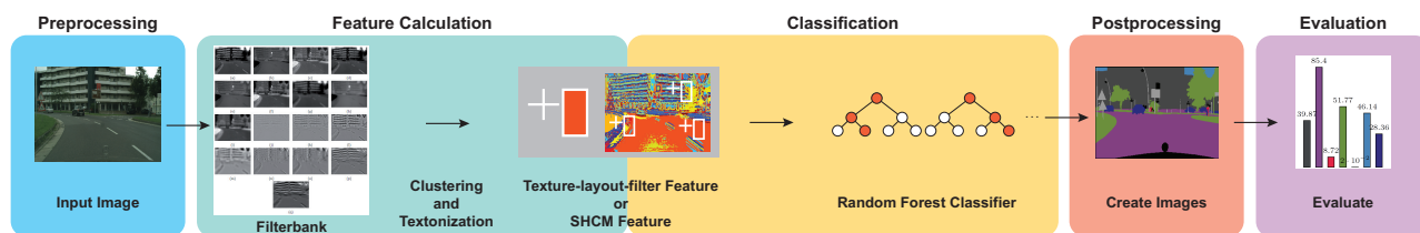
Fig. 1: Overview of our semantic segmentation system.
